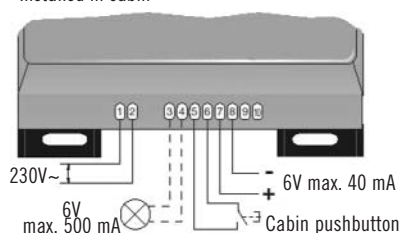
AKO-5404C Installed in cabin
