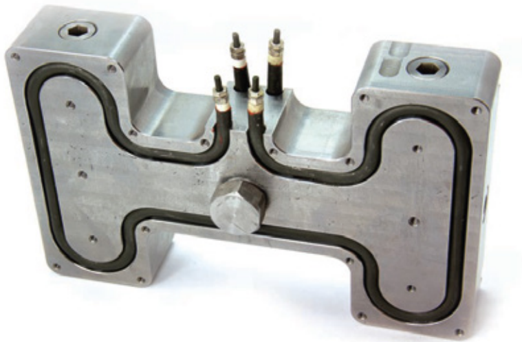
COLO ZONE 40mm EACH SIDE, CONNECTION THREA0EO STU0 M3X15L
